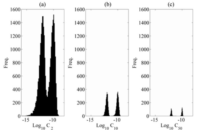
Fig. 2. Histograms of the series of the normalized sum of squares C_r (in logarithmic scale) of a 30s-cyclostationary process with \text{SNR} = 20 \text{ dB} and \text{DC} = 50\% for (a) r = 2 , (b) r = 10 , (c) r = 50 .
