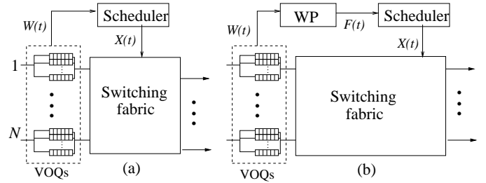
Fig. 1. Input queued switch architecture: (a) standard and (b) equipped with assisted scheduling.
