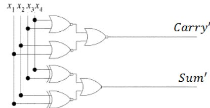
Figure 8. Gate level implementation of Design 2
