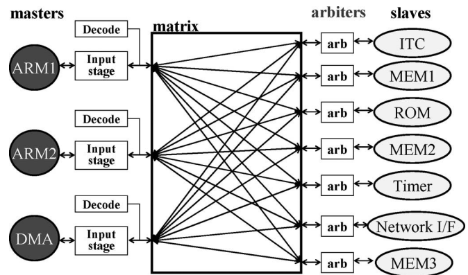
Fig. 1. Full bus matrix communication architecture.
