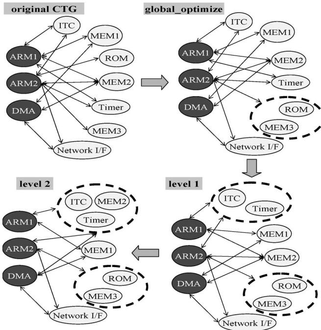
Fig. 7. Flow of clustering operations of best solution, for the example MPSoC system.
