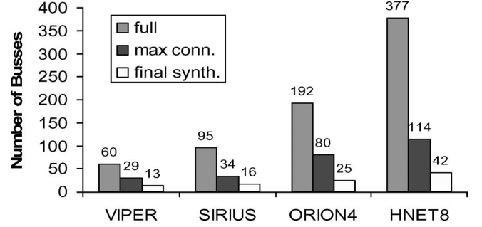
Fig. 15. Comparison of number of busses for MPSoC applications.
