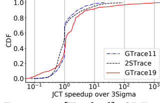
Figure 8: [Testbed] CDF of speedup: SLEARN vs 3Sigma.
