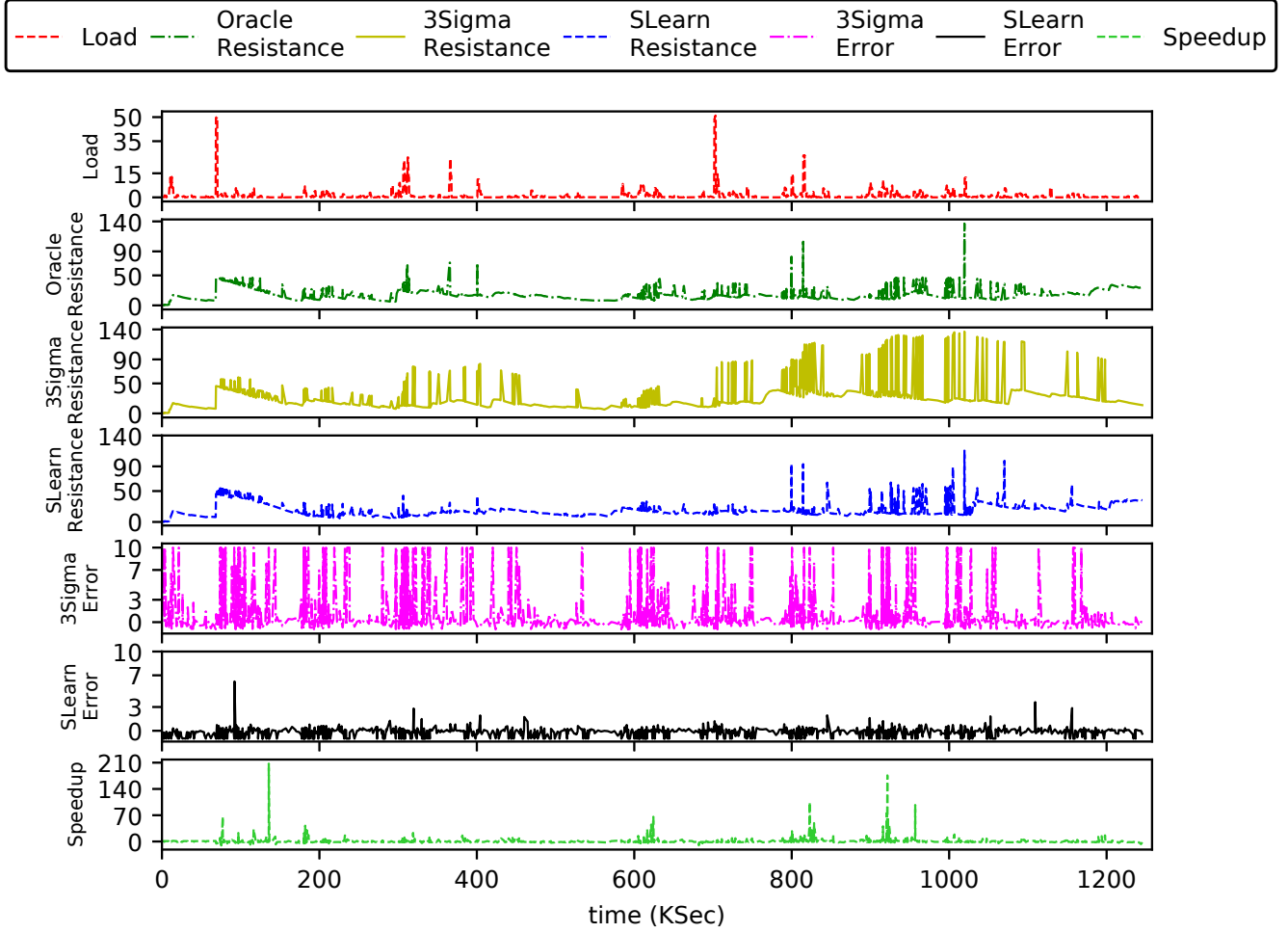
Figure 11: Correlation between load, resistance , estimation error and speedup for 2STrace.
