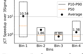
Figure 9: Performance breakdown down into the bins in Table 8.
