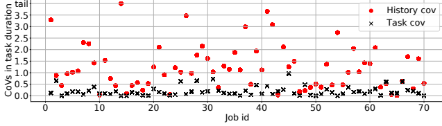
Figure 2: CoVs across time and space for 70 jobs selected randomly from the 2Sigma trace. The x-axis represents job ids in the order of their arrival.
