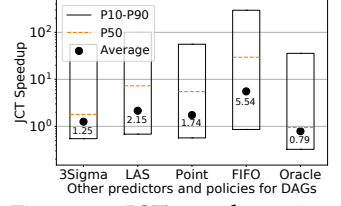
Figure 10: JCT speedup using SLEARN-DAG over baselines for GTrace19-DAG.
