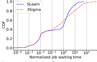
Figure 7: CDF of waiting times for wide jobs in GTrace11.
