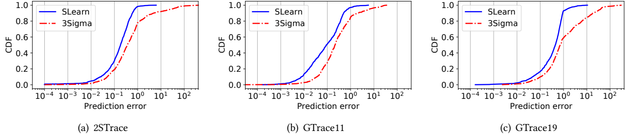
Figure 3: Job runtime prediction accuracy.
