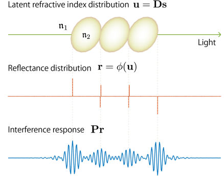
Fig. 4. Relationship among latent refractive index distribution \mathbf{u} , reflectance distribution \mathbf{r} and interference response \mathbf{Pr} .
