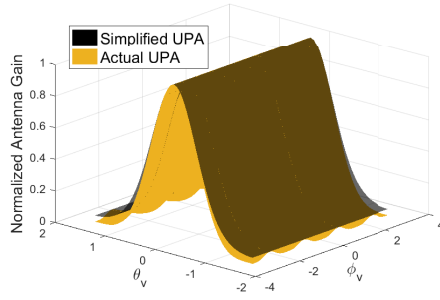
(a) Illustration of the simplified UPA and actual UPA.
