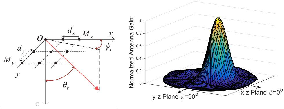
(a) The deployment of antenna elements in uniform planar array pattern. (b) Normalized antenna gain with \psi_v = \frac{\pi}{4} , \vartheta_v = \frac{\pi}{18} , 2d_x = 2d_y = \lambda_w = \frac{3 \times 10^8 \text{ m/s}}{28 \text{ GHz}} , and M_x = M_y = 4 .
