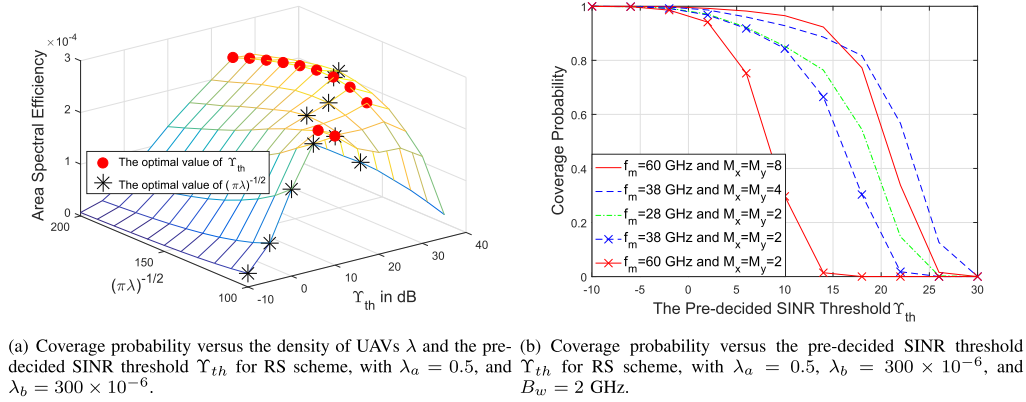
Fig. 7. The performance of ASE and different carrier frequencies.
