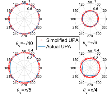
(b) Normalized antenna gain versus \psi_v with different \theta_v .
