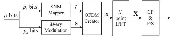
Fig. 1. System model of OFDM-SNM.
