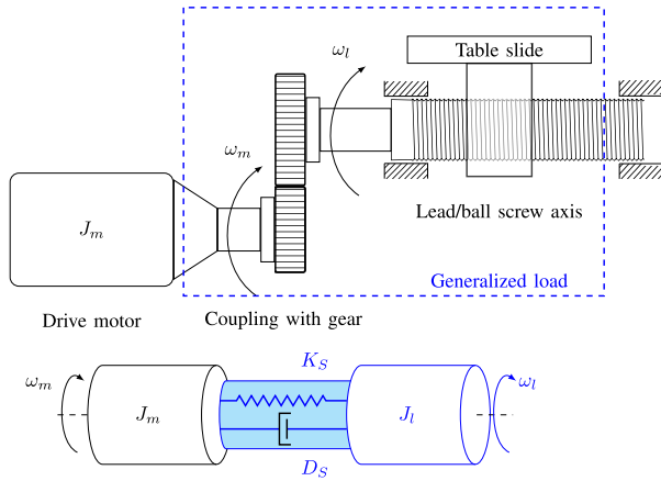
Fig. 1. Correspondence between mechanical drive-train and single-axis machine-tool systems. The angular velocities of the motor and the load are denoted by \omega_m and \omega_l , respectively.
