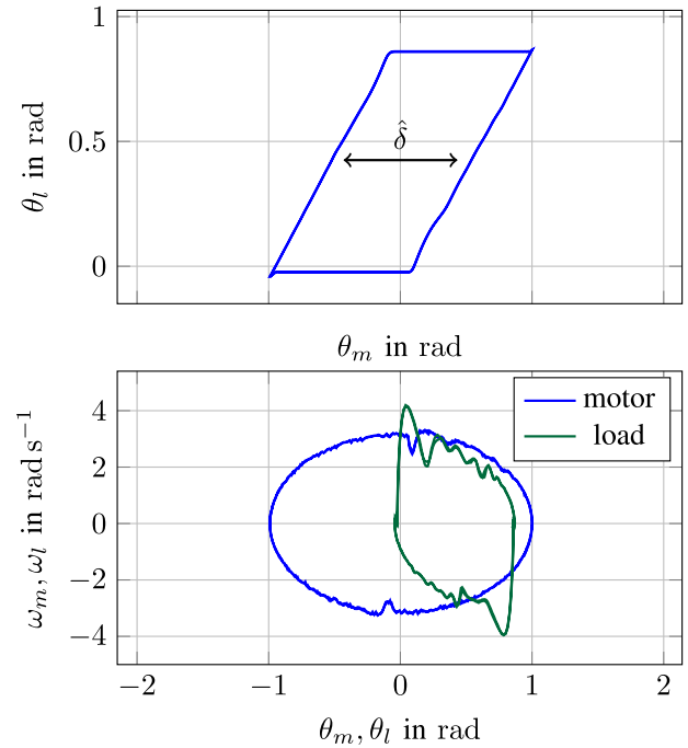
Fig. 16. Backlash hysteresis (top) and phase portraits for the motor and load (bottom) during Test 0A.
