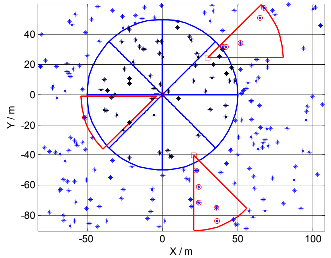
FIGURE 2. The simulated network scenario.
