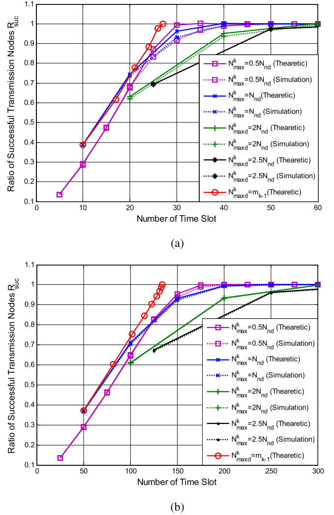
FIGURE 7. Ratio of successful transmission nodes R_{suc} for different N_{\max}^k in successive periods of the RA phase. (a) Ratio of successful transmission nodes R_{suc} with N_{nd} = 10 . (b) Ratio of successful transmission nodes R_{suc} with N_{nd} = 50 .
