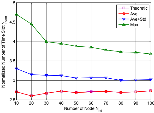
FIGURE 11. Total number of time slots in a RA phase.
