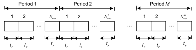
FIGURE 6. Detailed timing of the RDMA protocol in RA phase.
