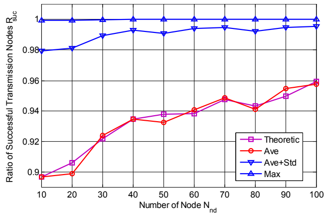
FIGURE 10. Ratio of successful transmission nodes R_{suc} .
