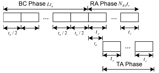
FIGURE 4. Time domain observation of the proposed scheme.
