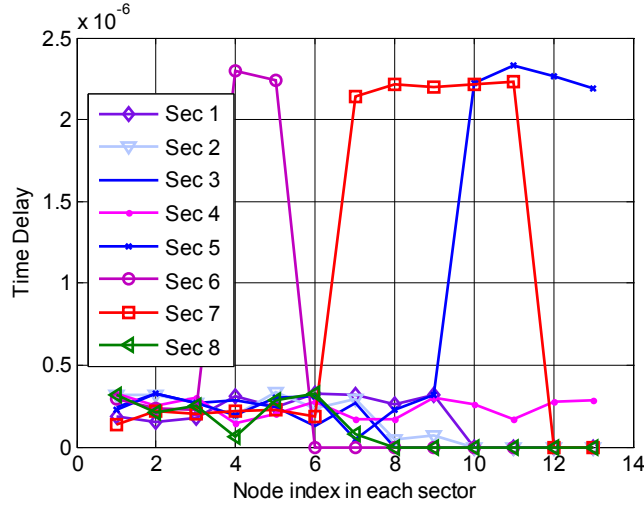
FIGURE 5. Time delay data obtained by the NC.
