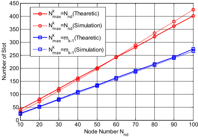
FIGURE 8. Number of slots required for successful transmission of all nodes in an interested sector.
