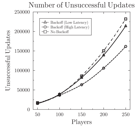
FIGURE 7. Unsuccessful Updates (Threshold = 60).
