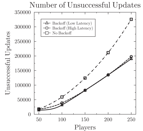
FIGURE 3. Unsuccessful Updates (Threshold = 30).
