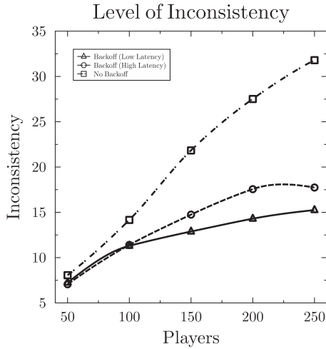
FIGURE 4. Level of Inconsistency (Threshold = 30).
