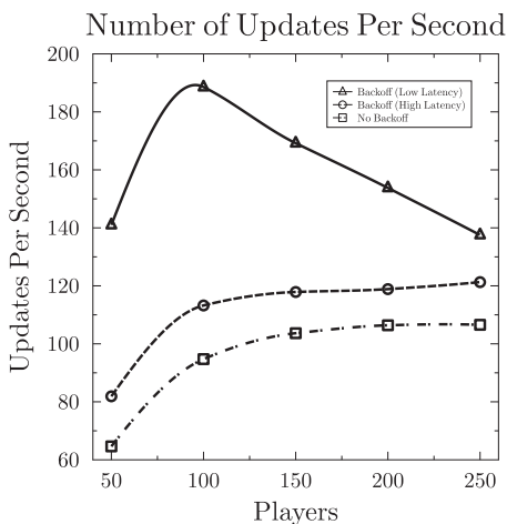
FIGURE 6. Message Throughput (Threshold = 30).
