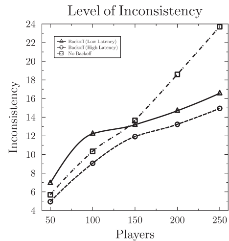
FIGURE 8. Level of Inconsistency (Threshold = 60).
