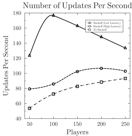
FIGURE 10. Message Throughput (Threshold = 60).
