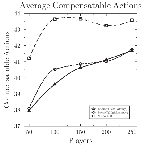
FIGURE 9. Average Compensatable Actions (Threshold = 60).
