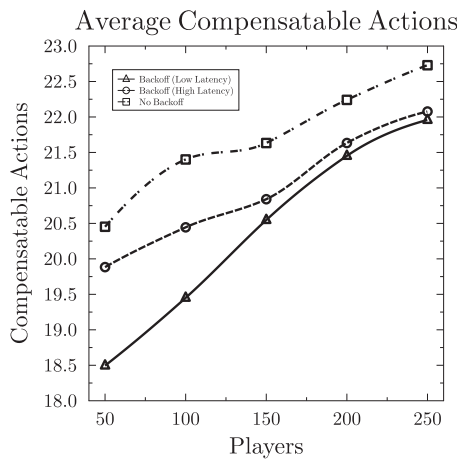
FIGURE 5. Average Compensatable Actions (Threshold = 30).
