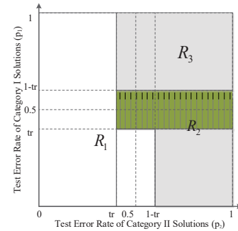
Fig. 6. The reliability configuration of the FNN constructed by the test errors p_1 and p_2 for estimating the uncertainty of the prediction.
