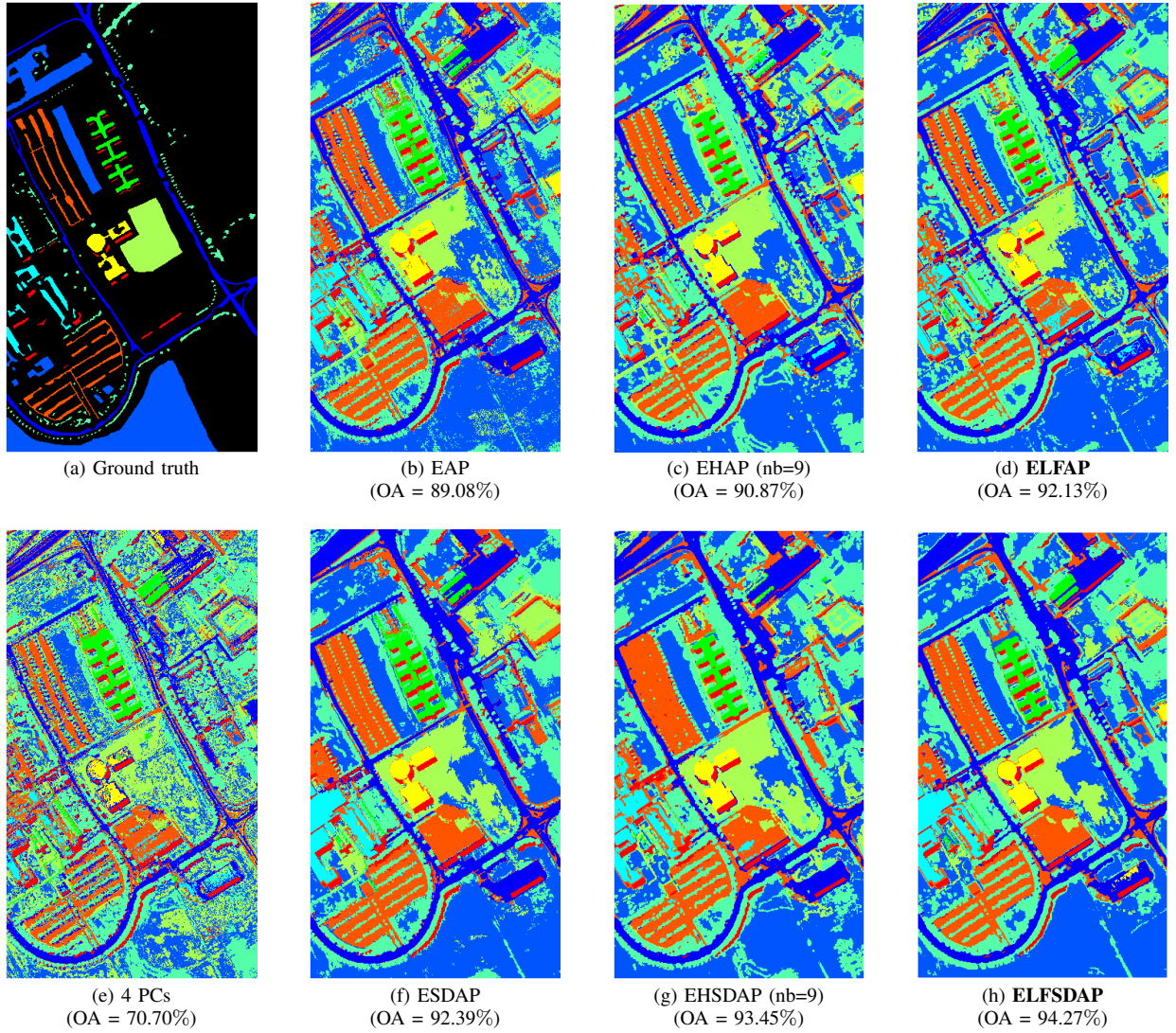
Fig. 6. Classification results of the Pavia University data obtained by different methods using a RF classifier with 200 trees.
