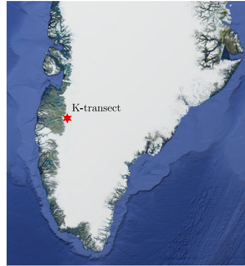
Fig. 13. Location of the K-transect test site in South-West Greenland ( 67^\circ 4' \text{ N} , 49^\circ 23' \text{ W} ).
