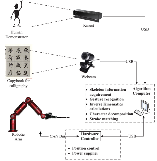
Fig. 9. The software implementation of the proposed approach.
