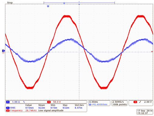
Fig. 19. Experimental results. Phase grid voltage (red trace, 50V/div) and injected current (blue trace, 1 A/div, THD= 4.5%) in case of the complete adopted SVM for the CSI7 topology.
