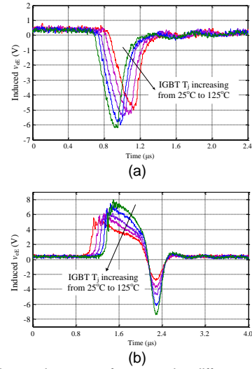
Fig. 10. Experimental v_{eE} waveforms under different IGBT T_j ( V_{dc}=1800 V, I_L=700 A and diode T_j=25^{\circ}\text{C} ). (a) Turn-off v_{eE} waveform comparison. (b) Turn-on v_{eE} waveform comparison.
