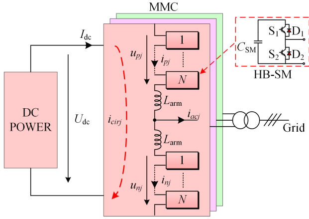
Fig. 1. Configuration of a Modular Multilevel Converter (MMC) system, where U_{dc} is the dc-link voltage, I_{dc} is the dc input current, u_{p(n)j} are arm voltages ( p = \text{upper arm}, n = \text{lower arm}, j = a, b, c ), i_{p(n)j} are arm currents, i_{cirj} is the circulating current, i_{acj} is the current of the phase j , L_{arm} is the arm inductor, C_{SM} is the sub-module (SM) capacitor, N is the number of SM per arm and HB-SM denotes a half-bridge SM.
