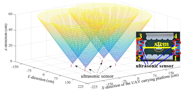
Fig. 9. Position distribution of ultrasonic sensors.
