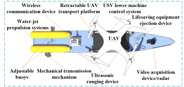
Fig. 2. Structure composition of the coupled USV-UAV platform.
