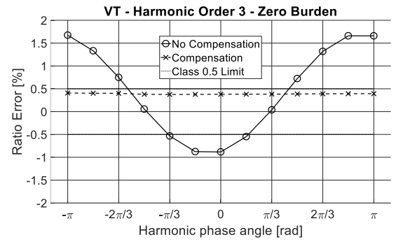
Fig. 10. Ratio error of the VT, with fundamental component of 120 %, third harmonic of 1 %, zero burden, with and without compensation
