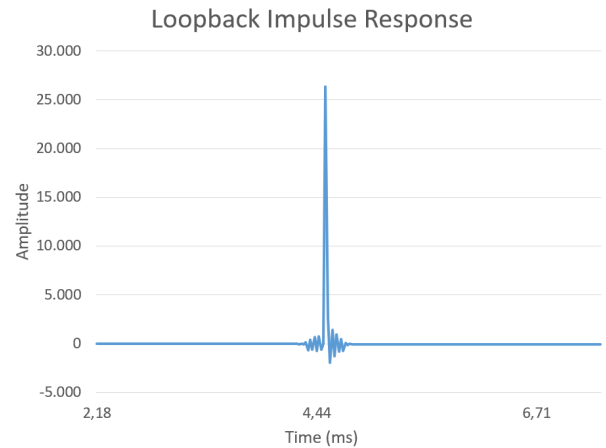
Figure 12. Loopback impulse response of the QS.
