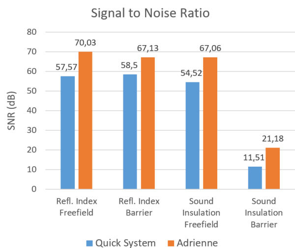
Figure 21. SNR obtained in the comparison measurements between the Adrienne system and the Quick system.
