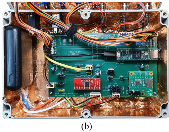
Figure 8. (a) Inside the main unit; (b) PCB main board.
