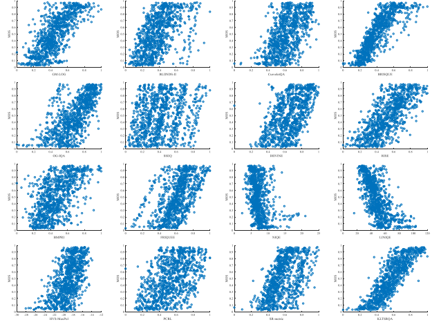
Fig. 13. Scatter plots of different NR-IQA metrics on QADS.
