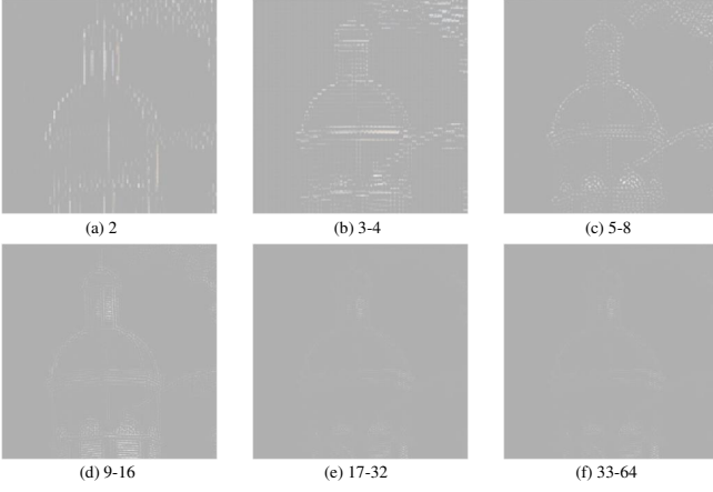
Fig. 6. Difference maps between the adjacent reconstruction results shown in Fig. 5. These difference maps are exactly the results reconstructed by the spectral components whose indexes are shown below each image.
