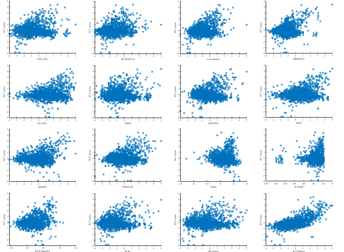
Fig. 11. Scatter plots of different NR-IQA metrics on RealSRQ.
