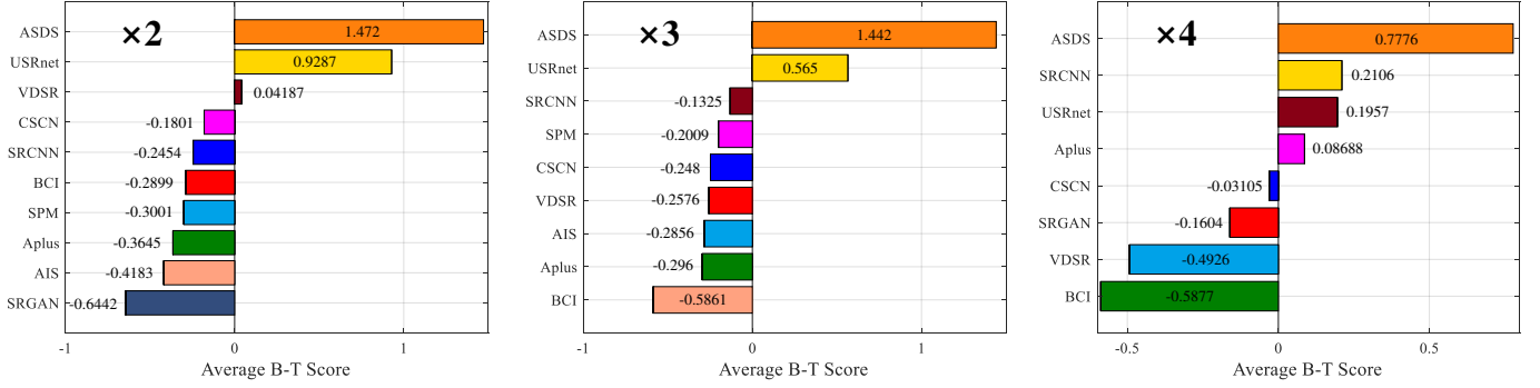
Fig. 2. Average B-T scores of different SISR algorithms at each scaling factor.
