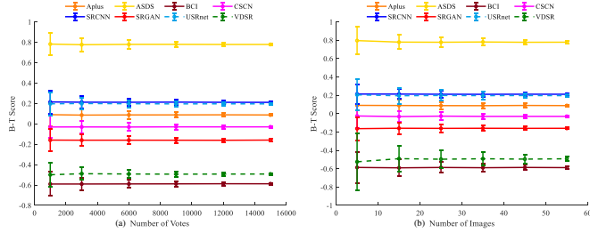
Fig. 3. Convergence analysis on the number of votes and images at scaling factor \times 4 .
