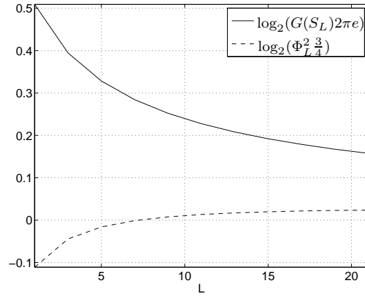
Fig. 2. The terms \log_2(G(S_L)2\pi e) and \log_2(\Phi_{L/4}^2 \frac{3}{4}) as a function of the dimension L . Both terms converge to 0 in the limit as L \rightarrow \infty . Notice that \log_2(G(S_L)2\pi e) > \log_2(\Phi_{L/4}^2 \frac{3}{4}) in the range shown.
