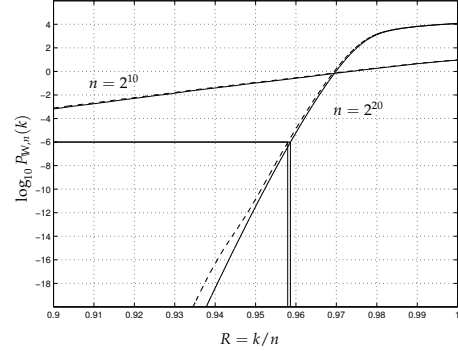
(b) binary-input AWGN channel with E_s/N_0 = 5.00 dB
