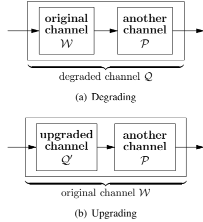
Fig. 3. Degrading and upgrading a channel \mathcal{W}
