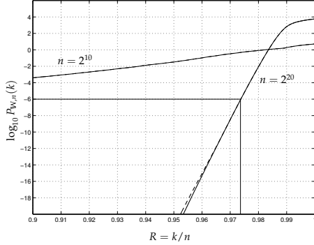
(a) Binary symmetric channel BSC(0.001)
