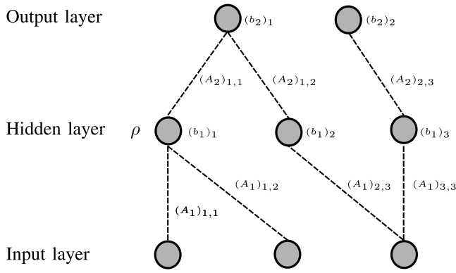
Fig. 1. Assignment of the weights (A_\ell)_{i,j} and (b_\ell)_i of a two-layer network to the edges and nodes, respectively.
