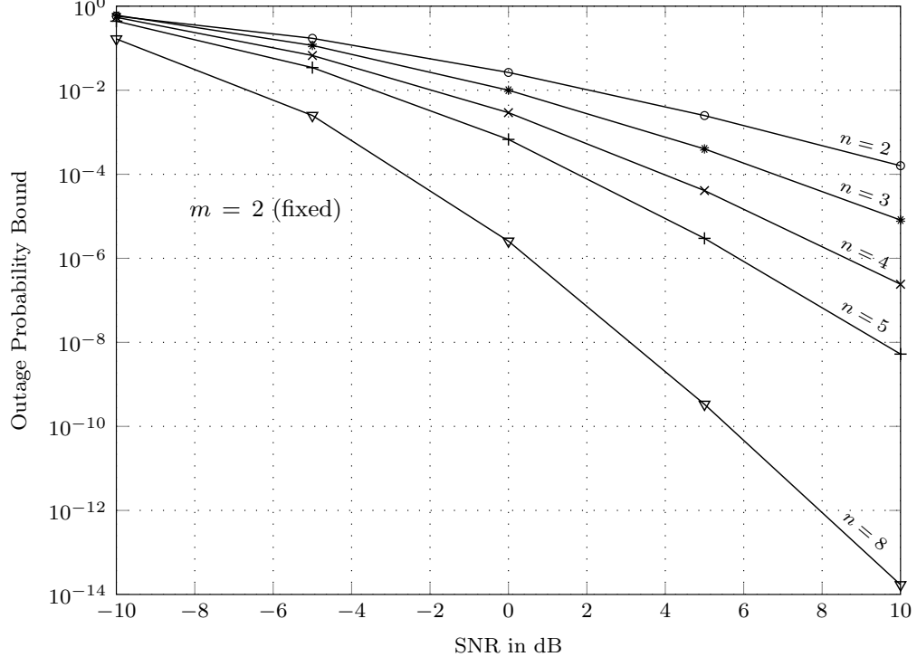
Fig. 6: Upper bound (Eq. (15)) for outage probability of a coherent MIMO IID Rayleigh channel with CSIT and m = 2 (fixed). This figure is a corrected version of the Fig. 9 in [1].
