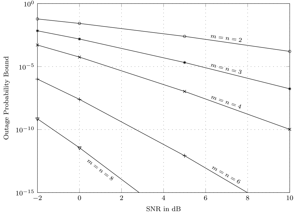
Fig. 7: Upper bound (Eq. (16)) for outage probability of a coherent MIMO IID Rayleigh channel with CSIT and m = n . This figure is a corrected version of the Fig. 10 in [1].
