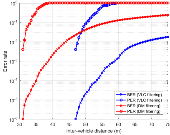
Fig. 10. BER and PER evolution against the V2V distance by steps of 50 cm with both “VLC filtering” and “DM filtering”.
