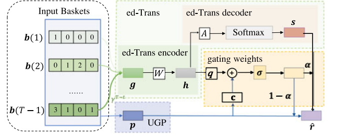
Fig. 2. M^2-gp^2t model architecture.
