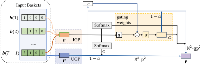
Fig. 1. M^2-p^2 and M^2-gp^2 model architectures.
