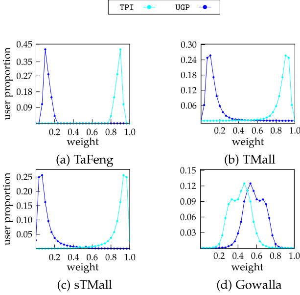
Fig. 4. Distributions of gating weights from M^2\text{-gp}^2t .
