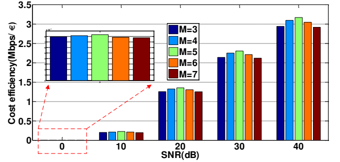
Fig. 9. Cost efficiency of 5G wireless backhaul networks with respect to the SNR over wireless channels and different number of gateways.
