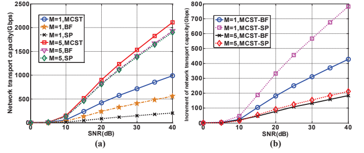
Fig. 11. Network transport capacity of 5G wireless backhaul networks with respect to the SNR over wireless channels and different number of gateways.
