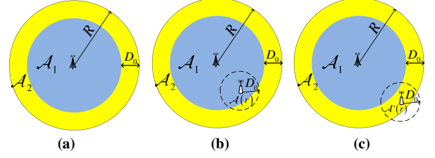
Fig. 3. Coverage regions of the MBS and SBSs
