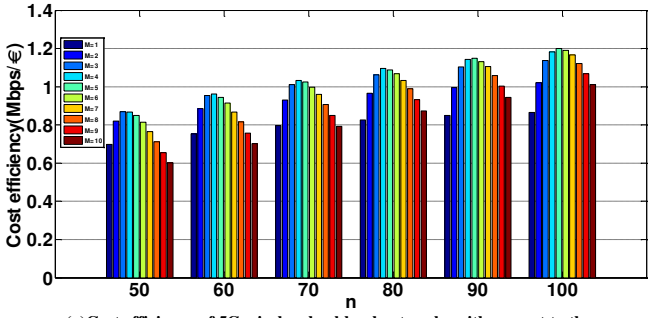
(a) Cost efficiency of 5G wireless backhaul networks with respect to the number of total SBSs with different number of gateways.
