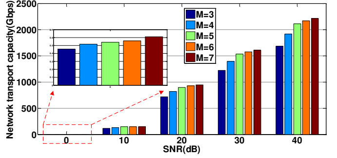
Fig. 8. Network transport capacity of 5G wireless backhaul networks with respect to the SNR over wireless channels and different number of gateways.
