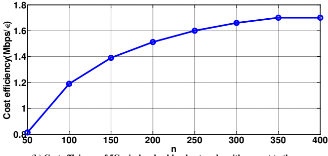
(b) Cost efficiency of 5G wireless backhaul networks with respect to the number of total SBSs.
