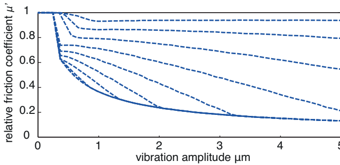
Fig. 14: The steady state relative coefficient of friction as a function of the vibrational amplitude calculated using the spring-slider model with the input parameters equal to those in Fig. 13 except that lateral recovery velocity of the skin was varied between 1.5 (top line) to 15 mm/s (lower line).
