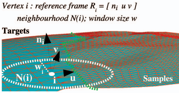
Fig. 3. 3D vertex neighborhoods N(i) .
