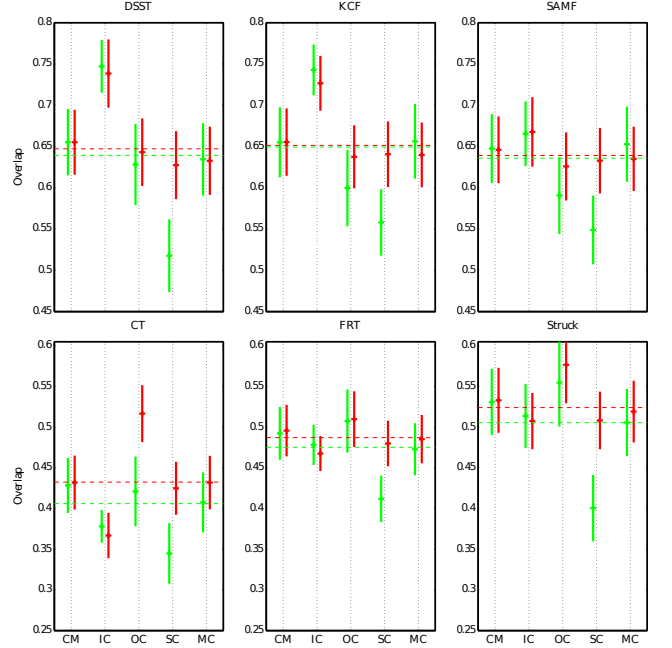
Fig. 6. The mean and variance of estimators that apply per-frame (green) and per-sequence (red) visual attribute annotation. The dashed lines show average performance on the dataset. The abbreviations CM, IC, OC, SC, and MC are used for camera motion, illumination change, occlusion, scale change and motion change, respectively.
