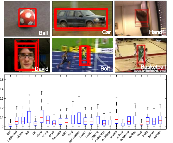
Fig. 4. Examples of the diversity of bounding box annotations for different images (top) and box plots of per-sequence distribution of ground truth overlaps.
