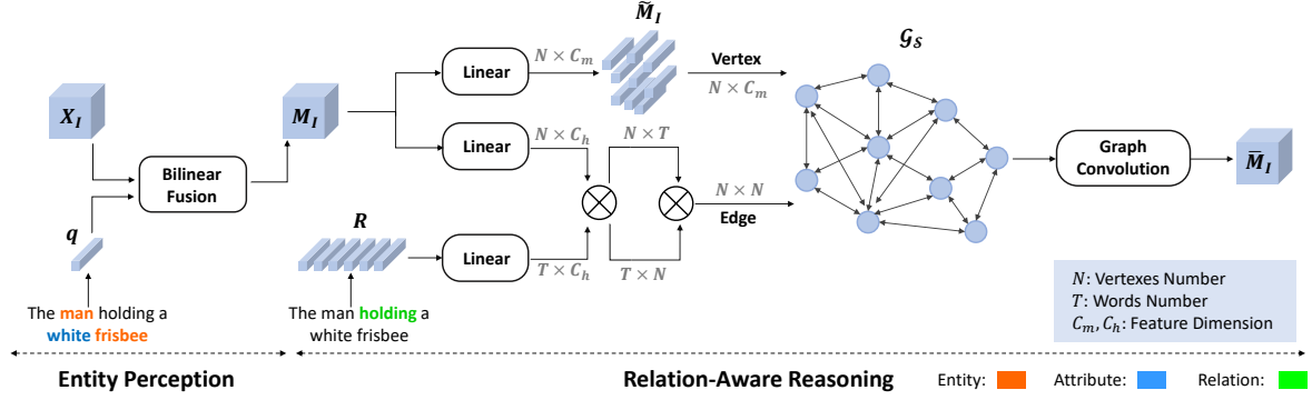
Fig. 3. Illustration of our CMPC-I module which consists of two stages. First, visual features X_I are bilinearly fused with linguistic features q of entity words and attribute words for Entity Perception (EP) stage. Second, multimodal features M_I from EP stage are fed into Relation-Aware Reasoning (RAR) stage for feature enhancement. A multimodal fully-connected graph \mathcal{G}_S is constructed with each vertex corresponds to an image region on M . The adjacency matrix of \mathcal{G}_S is defined as the product of the matching degrees between vertexes and relational words in the expression. Graph convolution is utilized to reason among vertexes so that the referent could be highlighted during the interaction with correlated vertexes.
