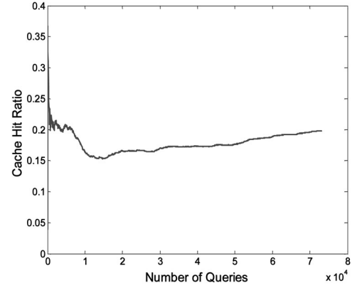
Fig. 3. Cache hit ratio on a single CGC peer with trace-driven query generator. Cache size is 1,024 KB.
