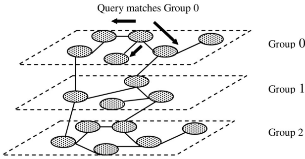
Fig. 1. Flooding in a multilayer P2P network.
