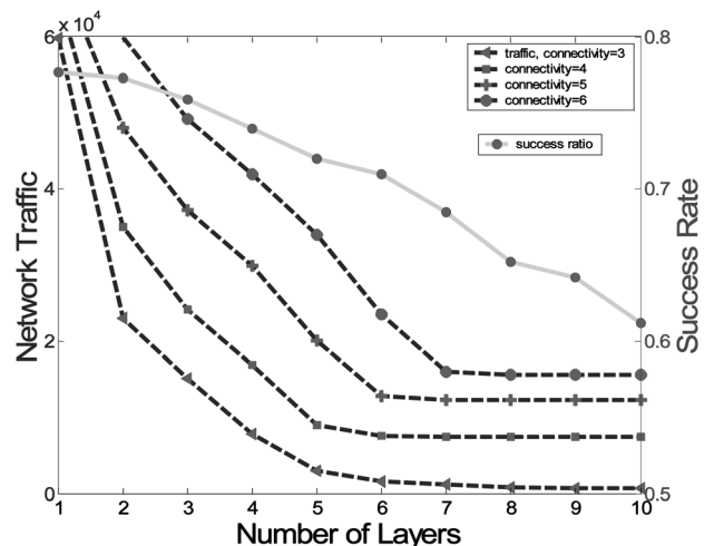
Fig. 15. Comparison for different number of layers.
