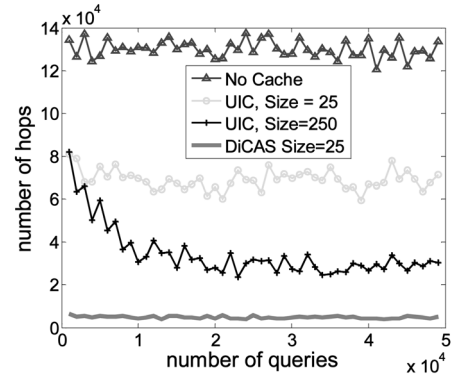
Fig. 12. Traffic comparison of UIC versus DiCAS.
