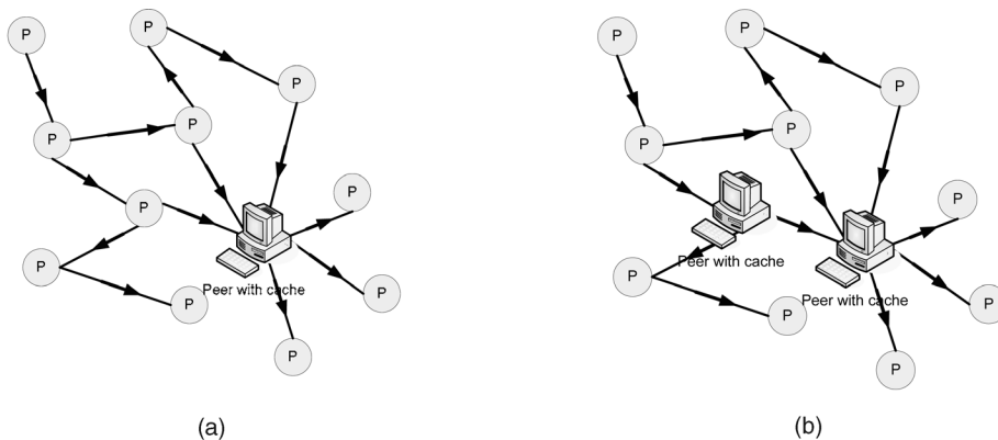
Fig. 4. CGC peers in Gnutella Network. In (a), a single CGC peer connected into Gnutella network, whereas in (b), two CGC neighboring peers connected to Gnutella network.
