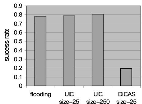
Fig. 13. Success rate comparison: UIC versus DiCAS.
