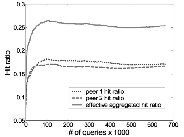
Fig. 6. Aggregate cache hit ratio in the twin CGCs experiment. The cache size on each CGC is 64K.
