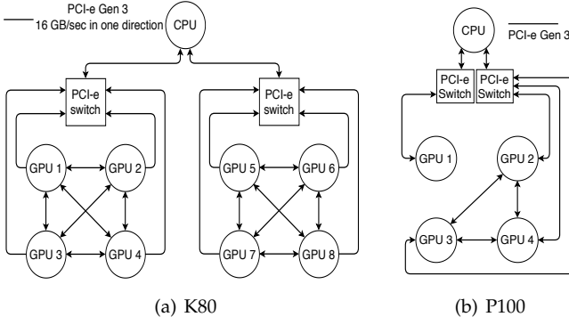
Fig. 6. Interconnection topology in a) K80, and b) P100
