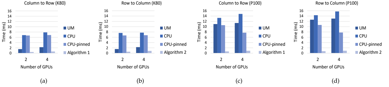
Fig. 4. Latency (in ms) of partitioning a matrix of dimensions (k = 40, n = 2^{16}) via four different approaches on NVIDIA TESLA K80 and NVIDIA TESLA P100. UM: unified memory. CPU: partitioning on CPU. CPU-pinned: partitioning on CPU but with pinned memory.
