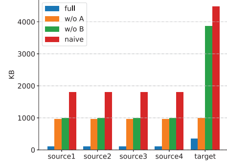
Fig. 4: Ablation study for optimization methods
