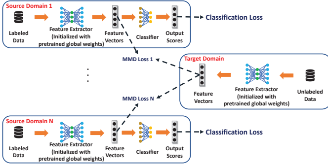
Fig. 3: A sketch of our federated multi-source domain adaptation framework (fine-tuning phase).
