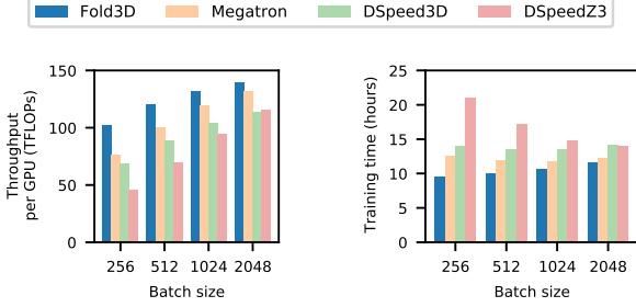
(b) FOLD3D achieved larger improvement over baselines under smaller batch size.
