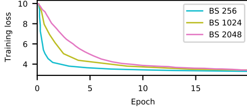
(a) BS means batch size. Model converges slower when using larger batch sizes.
