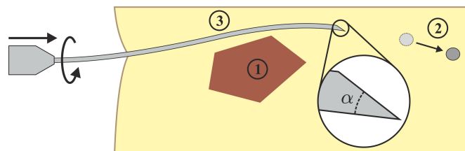
Fig. 1. Flexible needle with an asymmetric (bevel) tip can be used to steer around obstacles ①. Steering is accomplished by a combination of insertion and rotation at the base of the needle. Target motion ② may occur during needle insertion, and this affects targeting accuracy. ③ Single needle rotation results in the needle having a double-bend shape. The bevel angle is denoted by \alpha .
