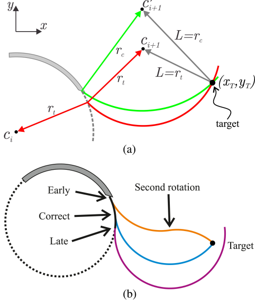
Fig. 9. (a) Variation in experimental conditions between insertions causes change in the radius of curvature of the needle r_t . Choosing the control radius r_c larger than the expected needle radius of curvature r_t results in an early rotation around the center c'_{i+1} . (b) Early needle rotation is corrected by performing additional rotations (orange). No additional rotation is required if the needle rotates at the correct instance (blue). If needle rotation is done late, then the target cannot be reached by performing additional rotations (purple).
