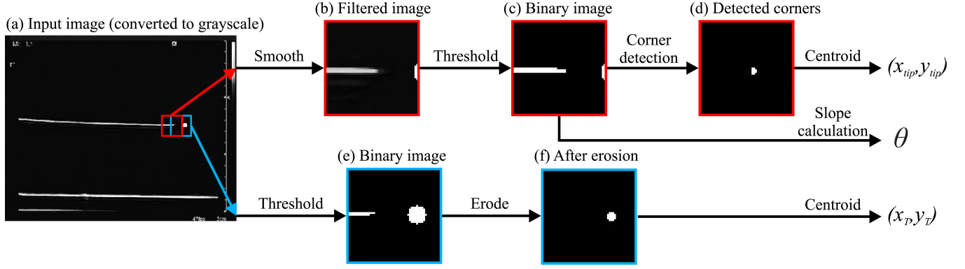
Fig. 11. Schematic shows the image processing algorithm applied to determine the needle tip position (x_{tip}, y_{tip}) and tip slope \theta (red window) and target position (x_T, y_T) (blue window). (a) Input is an ultrasound image which is converted to grayscale. (b) Grayscale image is smoothed to filter out artifacts. (c) Threshold is then applied to produce a binary image. (d) Harris corner detection is applied, and then, the centroid is calculated in the output image to detect the needle tip position. (e) Binary images are acquired after performing a threshold to detect the target position. (f) Erosion is used to filter out artifacts around the target, and then, the centroid of the image is calculated to determine the target location. This algorithm is also used for CCD camera images, but an additional processing step is applied. The image is inverted after applying the threshold.
