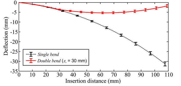
Fig. 7. Experimental needle tip deflection (mean) for the single-bend and the double-bend case ( x_r is the distance at which rotation is performed). In both cases, five insertions are performed, and the standard deviation \sigma is shown by the error bars. The mean final tip deflection is -31.3 mm ( \sigma = 1.0 mm) and -1.8 mm ( \sigma = 0.7 mm) for the single-bend and double-bend case, respectively. The curves show the tracked needle tip positions during insertion.
