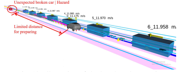
Fig. 10: Illustration of the benchmark scenario.
