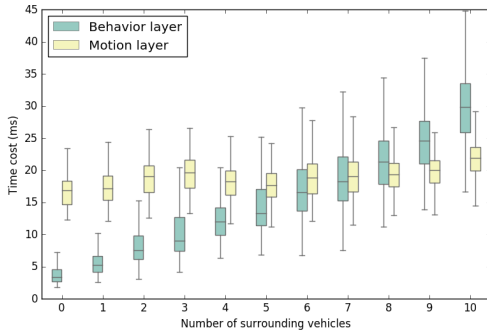
Fig. 12: Illustration of the computational time required by the proposed planning system w.r.t. the number of vehicles considered. Results for both the behavior layer and motion layer are presented.
