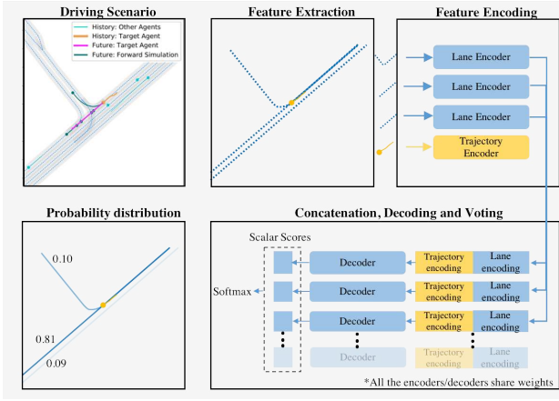
(a) Illustration of our lightweight network for estimating the semantic action (i.e., center-line) of other traffic participants.
