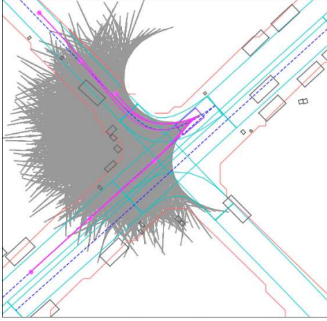
Fig. 3: Illustration of using semantic-level action to guide the exploration of the action space. Even with coarsely discretized control actions (e.g., three discretized longitudinal velocities and three lateral accelerations), the action space to be explored (gray) of a POMDP-based planner is huge during a multi-step look-ahead search, while most of the space explored is of low-likelihood. The situation is much worse when considering the multi-agent setting. After incorporating semantic-level action (e.g., pursuing center-lines with different aggressiveness) using predefined controllers, the exploration (purple) can be guided using domain knowledge. Although much of the exploration is pruned, the resulting exploration still faithfully captures the potential high-level decisions.
