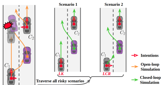
Fig. 5: Illustration of the CFB mechanism. Considering a case that the ego vehicle (purple) is considering a left lane-change. We use the open-loop simulation to get all possible future trajectories for all agents. Then, for each surrounding agent, we check whether there would be potential risks according to the simulated trajectories. For the critical agent ( C_1 ), we unfold all combinations of the possible intentions, and for the vehicle with low risk ( C_2 ), we directly employ the intention with maximum probability. As a result, the policy evaluation turns into an evaluation of the two scenarios. Interested readers may refer to [21] for more details.
