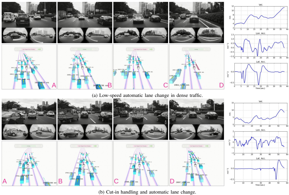
Fig. 16: Illustration of two automatic lane change scenarios in dense traffic. The visualization scheme is the same as in Fig. 15, and the difference is that the lane changes in Fig. 15 are upon user's request, while here, the lane changes are proposed by the planning system.
