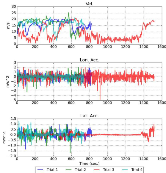
Fig. 14: Dynamic profiles for the four test drives. The time duration of the third trial is much longer than the others since the road is quite congested during the experiment. With the exception of a few rare cases, the vehicle's dynamics were kept within a comfortable range. For Trial-2 at around 590-th second, a lane-cancel behavior was executed in a risky situation, causing a relatively large lateral acceleration up to 1.60m/s^2 (actually still acceptable). At around 920-th second of Trial-3, the controlled vehicle made a hard brake ( -4.88m/s^2 ) because of a drastic deceleration of the leading vehicle.
