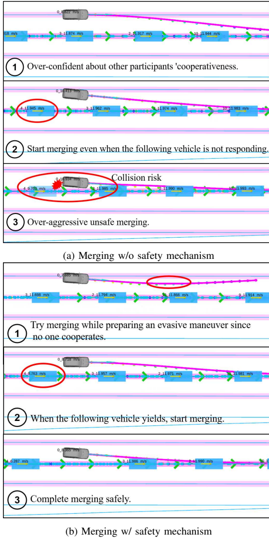
Fig. 11: Illustration of merging into dense traffic w/ and w/o safety mechanism. Note that the decoupled prediction-planning method is excluded here since it fails to conduct the lane change and gets trapped in the hazard. The best decision is visualized by the rainbow dots, while the corresponding trajectory is marked in purple .
