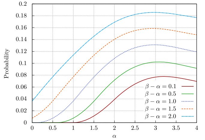
Fig. 12: The probability measure of paths satisfying (cs_3 = 0) \mathcal{U}^{[\alpha, \beta]}(cs_1 = 1) from marking m_0 = idle_1 idle_2 idle_3 .
