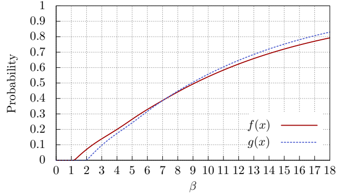
Fig. 11: The probability measure of paths satisfying \text{TRUE } \mathcal{U}^{[0, \beta]}(cs_1 = 1) from m_0 = idle_1 idle_2 idle_3 when write_1 is distributed according to truncated Erlang PDF f(x) = xe^{-20x}/400 over [0, 1] (mean value 0.1) or its symmetrical g(x) = f(1 - x) (mean value 0.9).
