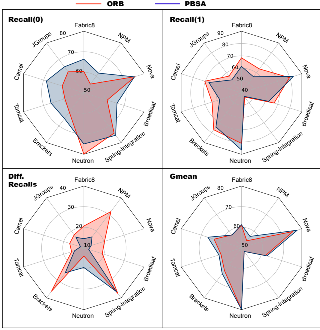
Fig. 7: Performance comparison for the average results of each metrics for ORB and PBSA classifiers.
