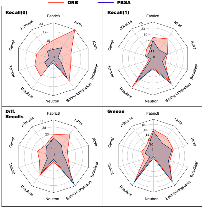
Fig. 8: Stability comparison for the average standard deviations through time of each metrics for ORB and PBSA classifiers.
