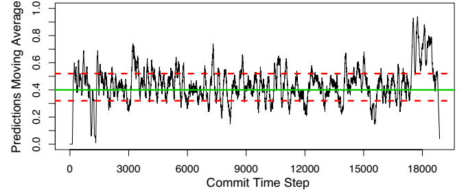
Fig. 5: Moving average of the predictions ( ws = 100 ) for the Tomcat dataset. Green line represents target moving average ( th ) and red dashed lines represent boundaries of the acceptable interval.
