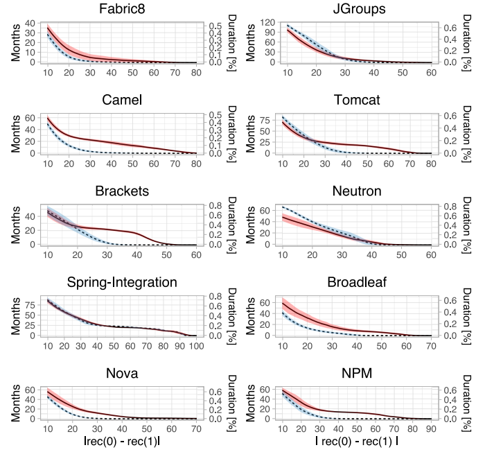
Fig. 9: Average number of months comprised in \Xi_l with l in the x axis. Blue area corresponds to the PBSA whereas the red one corresponds to ORB.
