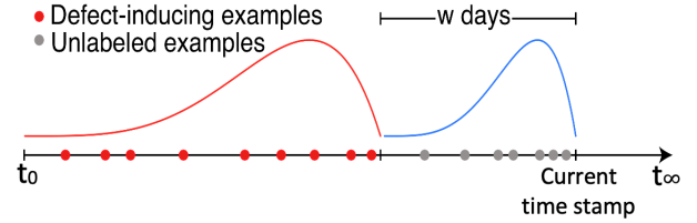
Fig. 6: PDF curves for picking an unlabeled example (blue curve) and for picking a defect-inducing example (red curve) for retraining the classifier.
