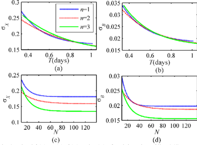
Fig. 8. Fitted f_M(T) , g_M(T) , f_T(N) and g_T(N) of each iteration of line 36#.
