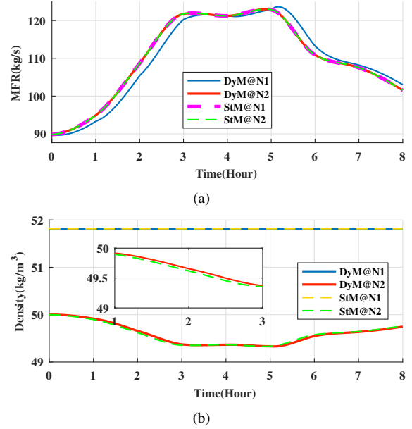
Fig. 4. Comparison between the static model (StM) and dynamic model (DyM) of gas flow. (a) The nodal MFR of the single pipeline with the static and dynamic model. (b) The nodal density of the single pipeline with the static and dynamic model.
