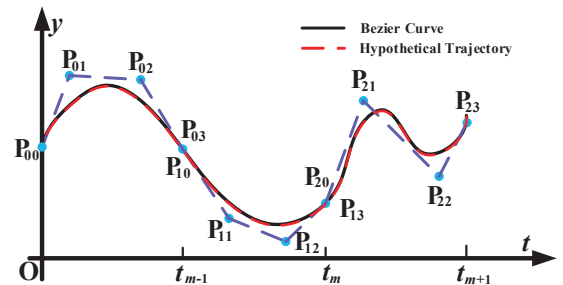
Fig. 1. The control points of Bernstein polynomials and the Bézier curve.
