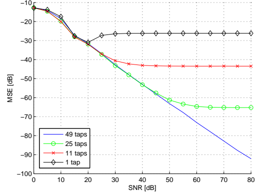
Fig. 9. MSE of the delays estimation versus SNR for different lengths of digital correction filter bank approximations.
