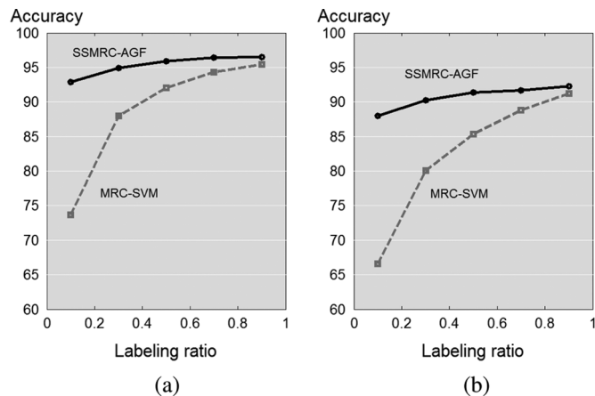
Fig. 8. Trend 2: Semi-supervised learning improves classification accuracy. Comparison of multiresolution classifiers. (a) Vehicle 1. (b) Vehicle 2.
