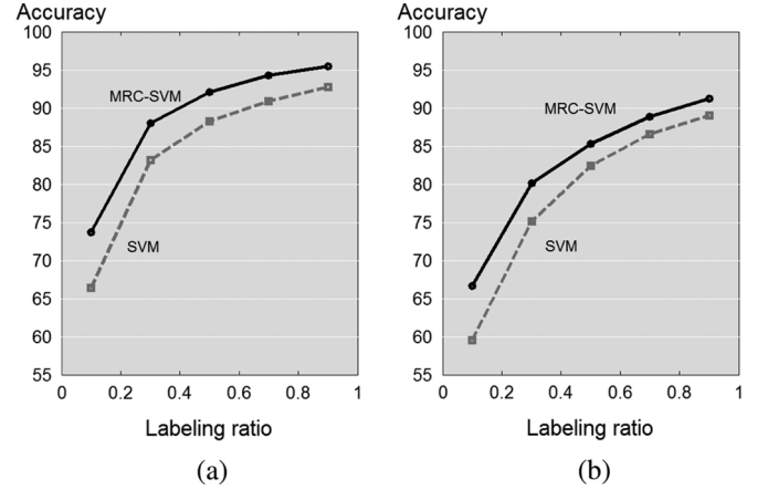
Fig. 6. Trend 1: Multiresolution framework improves classification accuracy. Comparison of supervised classifiers. (a) Vehicle 1. (b) Vehicle 2.
