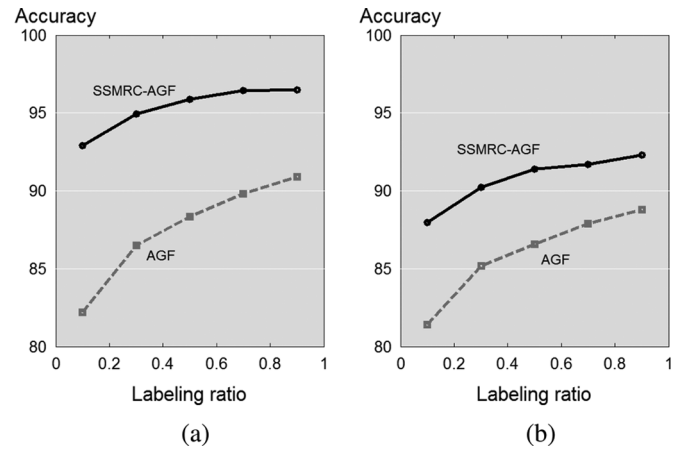
Fig. 7. Trend 1: Multiresolution framework improves classification accuracy. Comparison of semi-supervised classifiers. (a) Vehicle 1. (b) Vehicle 2.
