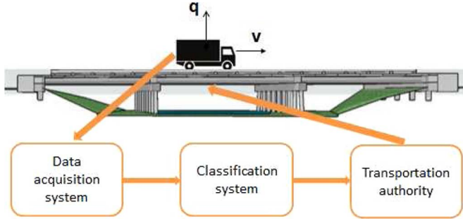
Fig. 1. Indirect bridge structural health monitoring system. Acceleration signals are collected from a moving vehicle and sent to a classification system, which identifies the bridge status and reports it to a transportation authority.
