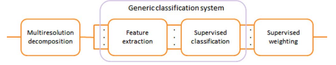
Fig. 2. Supervised multiresolution classification decomposes a signal into localized space-frequency subbands using a given multiresolution transform, followed by feature extraction and supervised classification in each subband, yielding a local classification decision. A supervised weighting algorithm combines all local decisions into a global decision.
