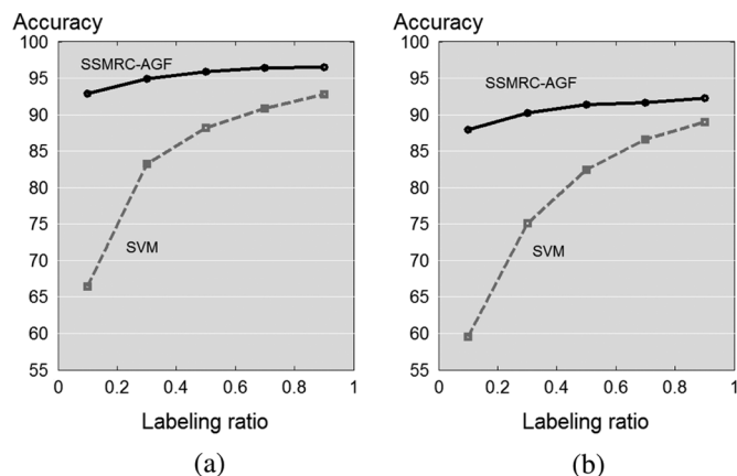
Fig. 9. Trend 3: Multiresolution framework with semi-supervised learning improves classification accuracy. (a) Vehicle 1. (b) Vehicle 2.
