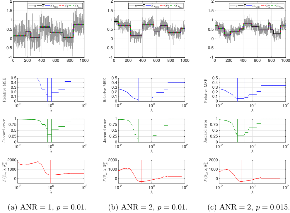
Figure 2: Illustration of the automated tuning of \lambda : Top: Data \mathbf{y} to which are superimposed true signal \bar{\mathbf{x}} and oracle signals \hat{\mathbf{x}}_{\lambda_{\text{MSE}}} (blue) and \hat{\mathbf{x}}_{\lambda_{\text{Jac}}} (green) obtained for \lambda_{\text{MSE}} and \lambda_{\text{Jac}} minimizing the MSE and the Jaccard error, together with estimated \hat{\mathbf{x}}_{\hat{\lambda}} (red) obtained from automated selection of \lambda . Second and third lines: relative MSE and Jaccard error as functions of \lambda . Vertical lines locate \lambda_{\text{MSE}} and \lambda_{\text{Jac}} . Bottom line: Criterion F (cf. (23)) as a function of \lambda . Automatically selected \hat{\lambda} is indicated by vertical red lines and is satisfactorily located in between the vertical lines indicating \lambda_{\text{MSE}} and \lambda_{\text{Jac}} . (left) p = 0.01 and ANR = 1, (middle) p = 0.01 and ANR = 2, (right) p = 0.15 and ANR = 2. For all configurations, \bar{x}_{\max} - \bar{x}_{\min} = 1 .
