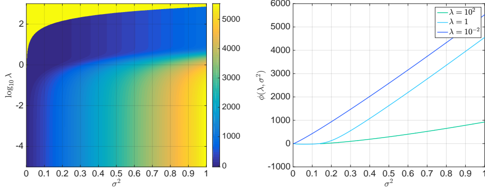
Figure 1: Illustration of \phi(\lambda, \sigma^2) for the hyperparameter setting \alpha_0 = \alpha_1 = 1 and 2\pi\sigma_0^2 = 10^4 .
