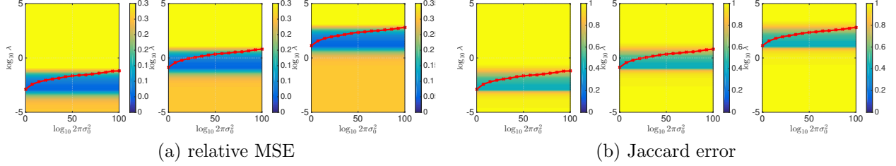
Figure 6: Estimation performance: RMSE and Jaccard error as functions of \lambda and \sigma_0^2 . The background displays the relative MSE (left) or Jaccard error (right) w.r.t. \lambda and \sigma_0^2 . We superimpose in red the estimate \hat{\lambda} , which a priori explicitly depends on the choice of the hyperprior \sigma_0^2 , is averaged over 50 realizations and displayed in red as a function of 2\pi\sigma_0^2 . From left to right: \bar{x}_{\max} - \bar{x}_{\min} = 0.1, 1 and 10 . For each configuration p = 0.01 , \text{ANR} = 1 . Choosing \log 2\pi\sigma_0^2 \in [0, 5] systematically leads to satisfactory estimates minimizing the relative MSE (left) or Jaccard error (right).
