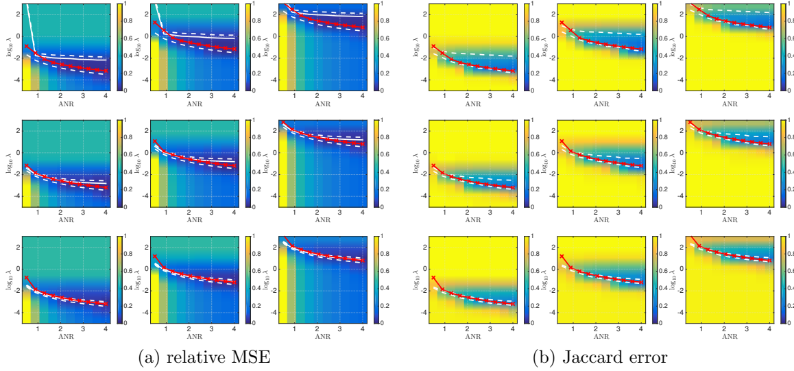
Figure 3: Estimation performance: RMSE and Jaccard error as functions of \lambda and ANR. The background displays the relative MSE (left) or Jaccard error (right) w.r.t. \lambda and ANR. We superimpose in red the estimate \hat{\lambda} (average over 50 realizations), as a function of the ANR, which is shown to satisfactorily remain within the range of oracles \lambda , delimited by dashed white lines and to closely follow oracle Monte Carlo average indicated by solid white lines (left: relative MSE, right: Jaccard error). From top to bottom: p = 0.005, 0.010 and 0.015 . From left to right: \bar{x}_{\max} - \bar{x}_{\min} = 0.1, 1 , and 10 .
