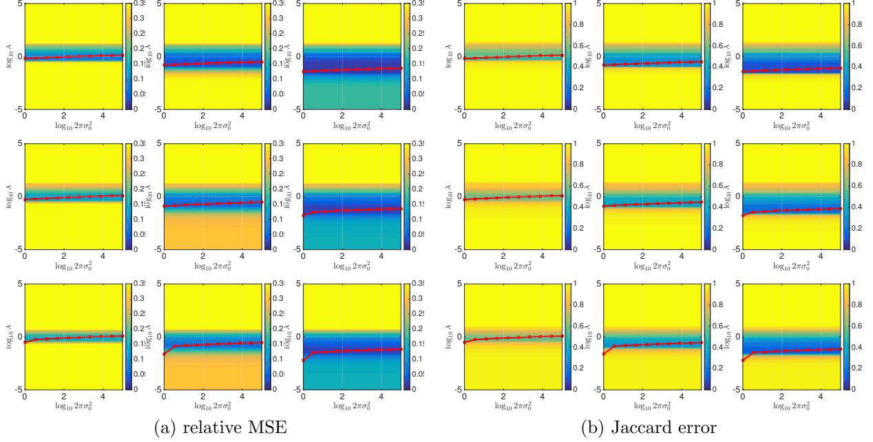
Figure 7: Estimation performance: RMSE and Jaccard error as functions of \lambda and \sigma_0^2 . The background displays the relative MSE (left) or Jaccard error (right) w.r.t. \lambda and \sigma_0^2 . We superimpose in red the estimate \hat{\lambda} , which a priori explicitly depends on the choice of the hyperprior \sigma_0^2 , is averaged over 50 realizations and displayed in red as a function of 2\pi\sigma_0^2 . Choosing \log 2\pi\sigma_0^2 \in [0, 5] leads to satisfactory estimation performance independently of p and the ANR. For each configuration \bar{x}_{\max} - \bar{x}_{\min} = 1 . From top to bottom: p = 0.005, 0.010 and 0.015 . From left to right: \text{ANR} = 1, 2 and 4 .
