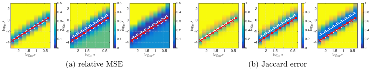
Figure 4: Estimation performance: RMSE and Jaccard error as functions of \lambda and \sigma . The background displays the relative MSE (left) or Jaccard error (right) w.r.t. \lambda and \sigma . We superimpose in red the estimate \hat{\lambda} (average over 50 realizations), as a function of \log_{10} \sigma , which is shown to satisfactorily remain within the range of oracles \lambda , delimited by dashed white lines and to closely follow oracle Monte Carlo average indicated by solid white lines (left: relative MSE, right: Jaccard error). For each configuration p = 0.01 and from left to right: \text{ANR} = 1, 2 and 4 . This illustrates that \hat{\lambda} leads to solutions with same performance as oracle \lambda and highlights that \hat{\lambda} varies linearly with \sigma^2 , as expected.
