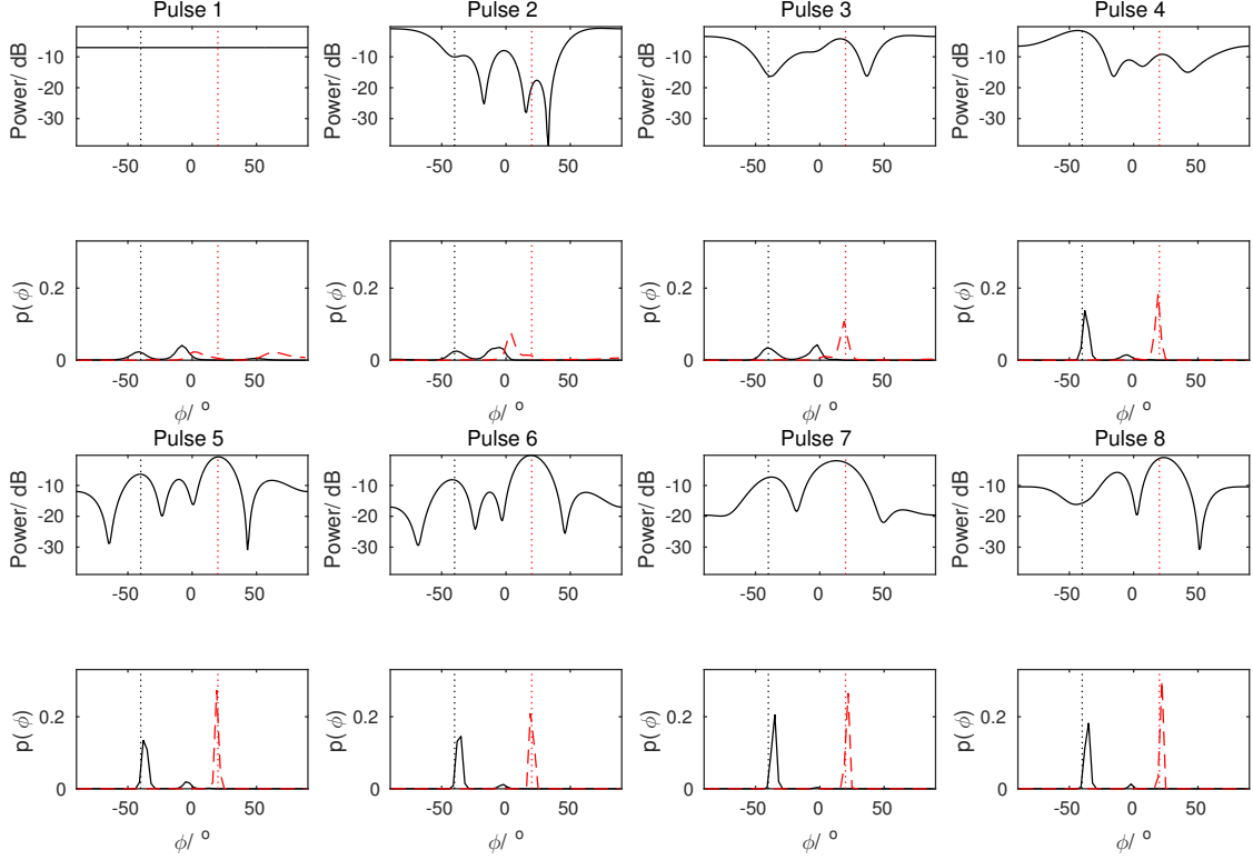
Fig. 6. Example of the first eight pulses of MMSE adaptive waveform design. Two targets located at -40^\circ and 20^\circ as indicated by the vertical dotted lines.
