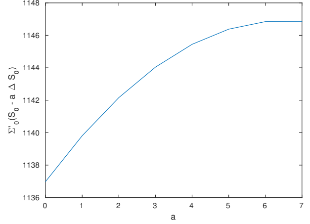
Fig. 8. Special case to show that the optimisation surface is not convex
