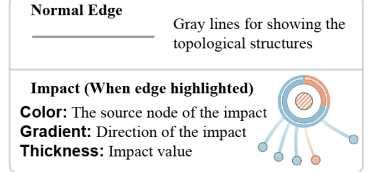
Fig. 7. Visual design of the local impact view. (a) The process of building k NN graph structures. (b) The visual encodings for nodes and edges.
