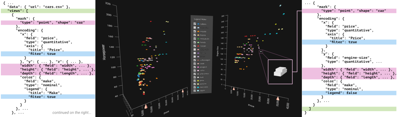
Fig. 12. An example of multiple linked views in <VRIA> and their corresponding vis config file (shortened for brevity). Any number of plots can be linked and changes to one of the filters or the legend will update the other views. This example also demonstrates the use of a custom mark. Custom marks can also be 3D models (e.g., glTF), which are nonetheless expensive to render, hence why we opt for a simpler mark for this example.
