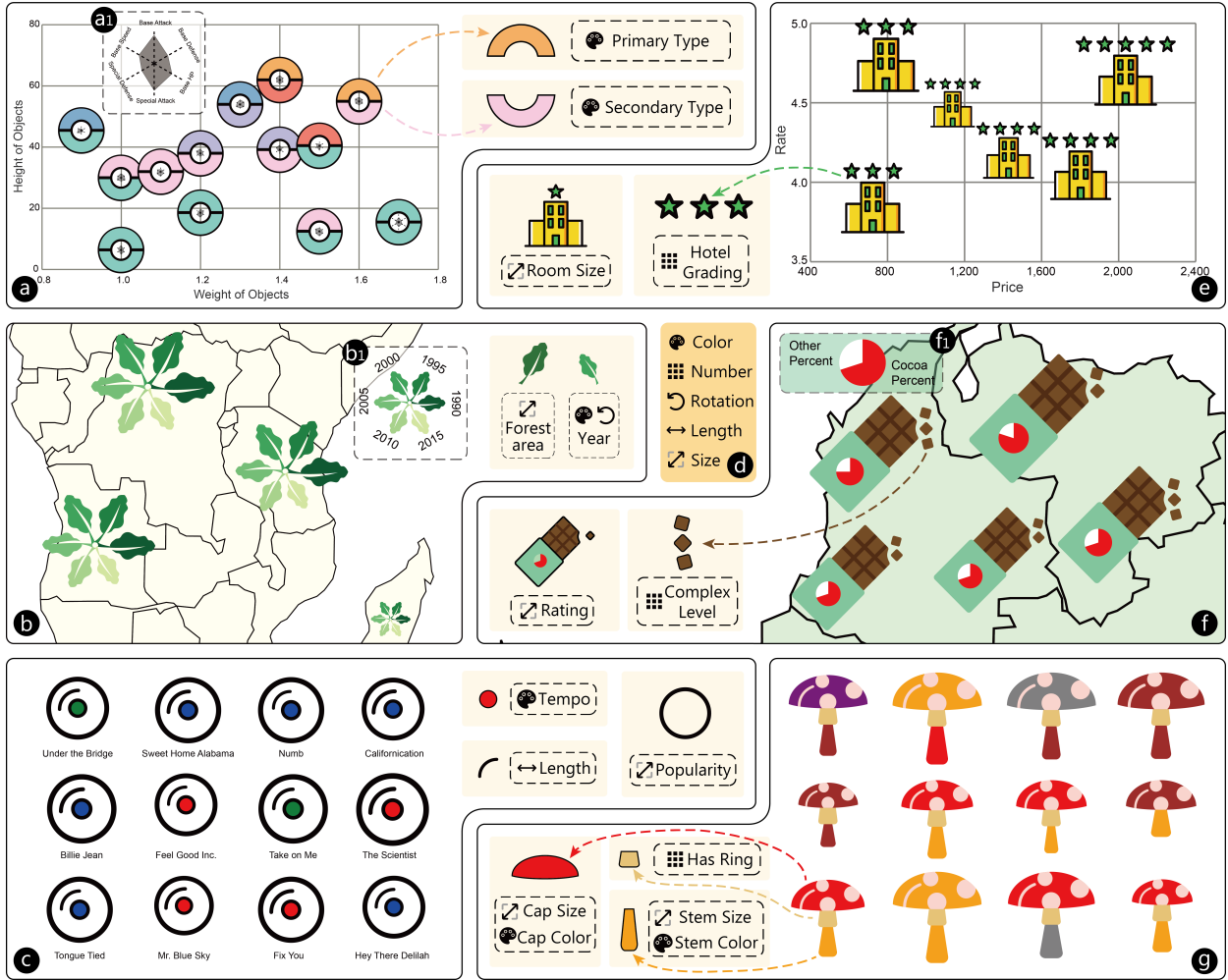
Fig. 1. Example MGVs generated by MetaGlyph: (a) several attributes of different pokemons; (b) forest area changes in different countries from 1995 to 2020; (c) display of various CDs; (e) multiple hotels' information arranged by price (x) and rate (y); (f) chocolates in different ratings placed on a map; (g) disparate mushrooms. The legends in (a1)(b1)(f1) are also generated by MetaGlyph. The center boxes with yellow backgrounds illustrate the data mappings for each glyph. Encoding channels are represented in icons and (d) shows the annotation. Dashed arrows are used to associate visual elements with the resulting visualizations.
